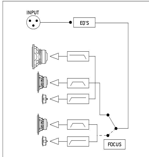
Diagramme mode FOCUS TRI06 Be.
