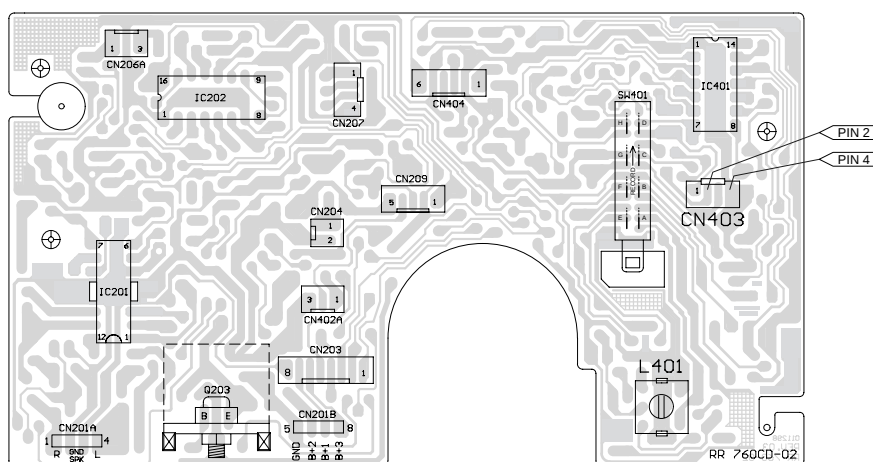
Amplifier Board
