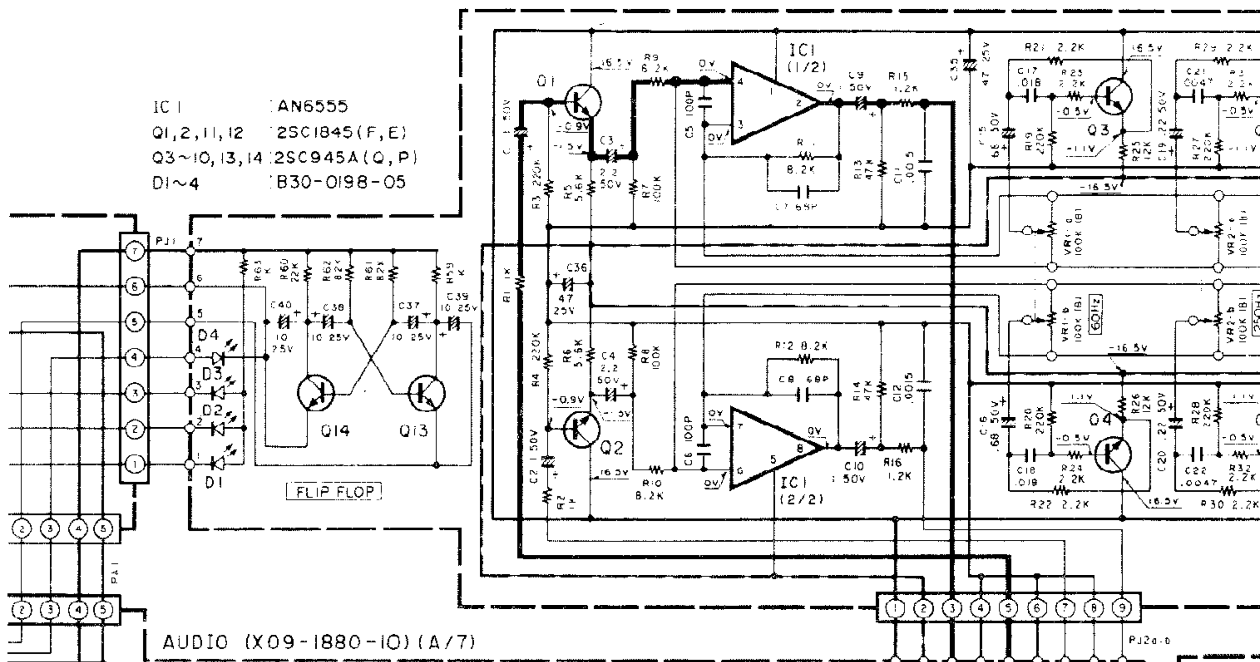
GRAPHIC EQ. (X11-1740-10)
