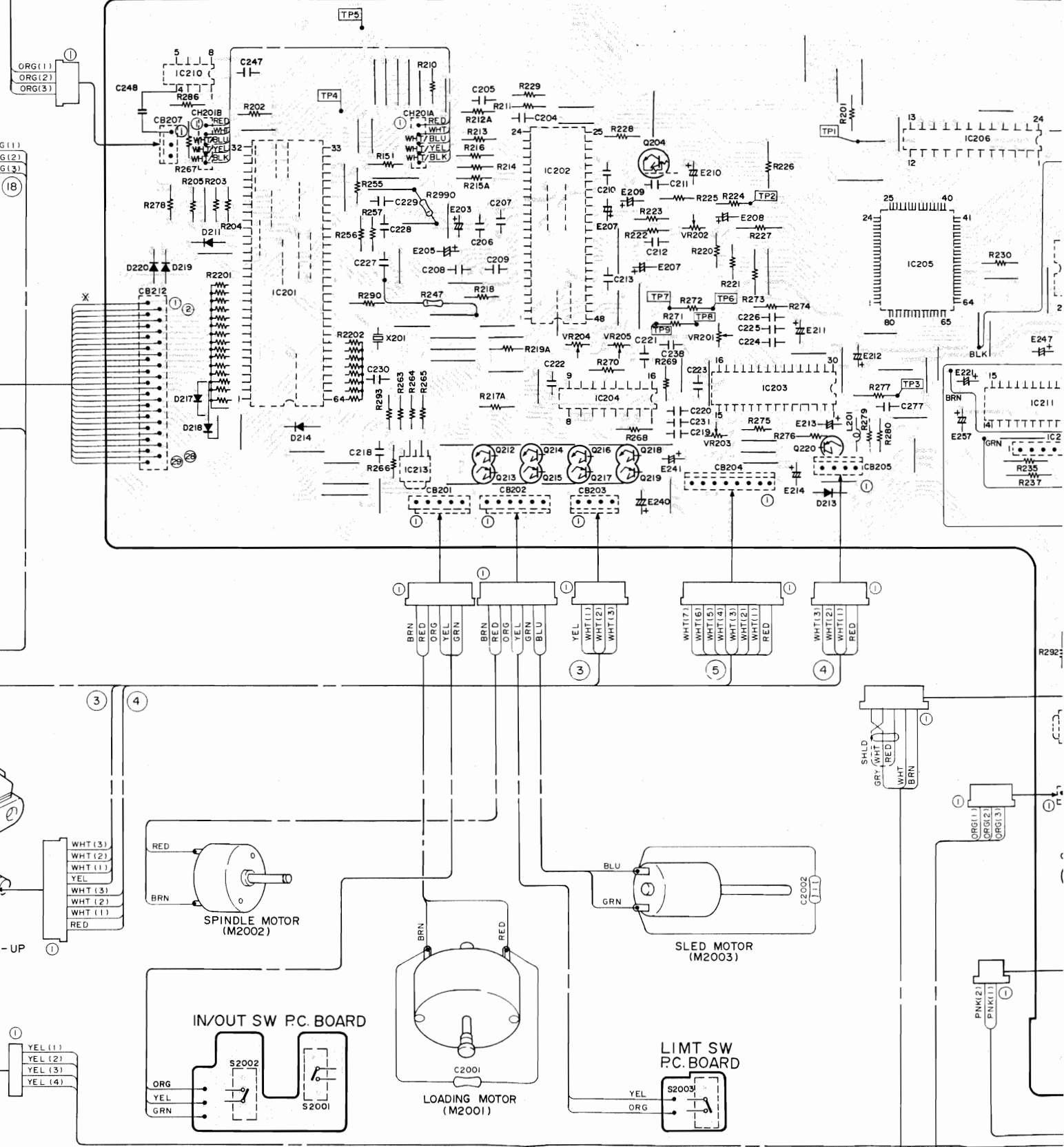
MAIN P.C. BOARD
