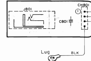
HEAD PHONE P.C. BOARD
