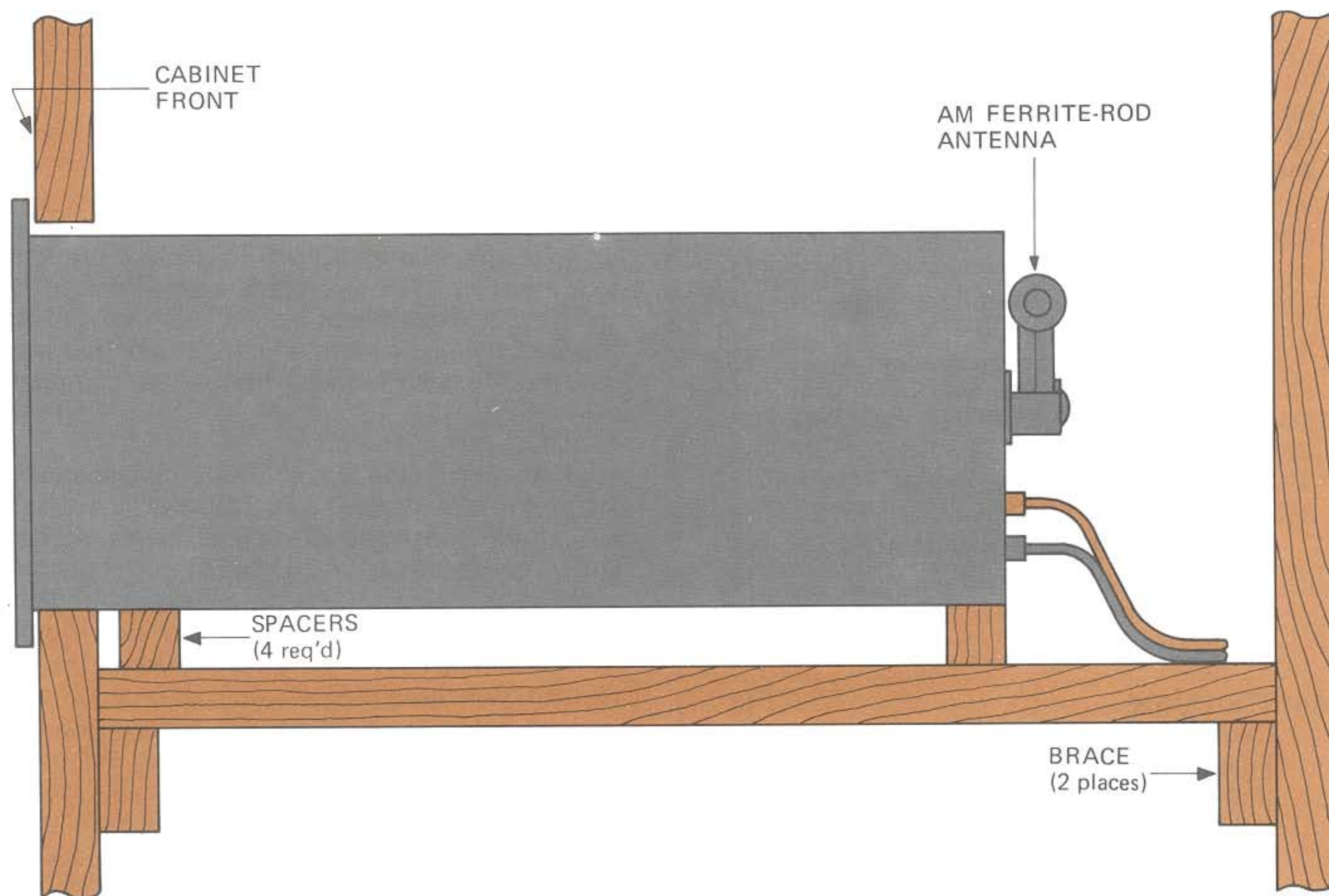
Figure 1. Custom Mounting
