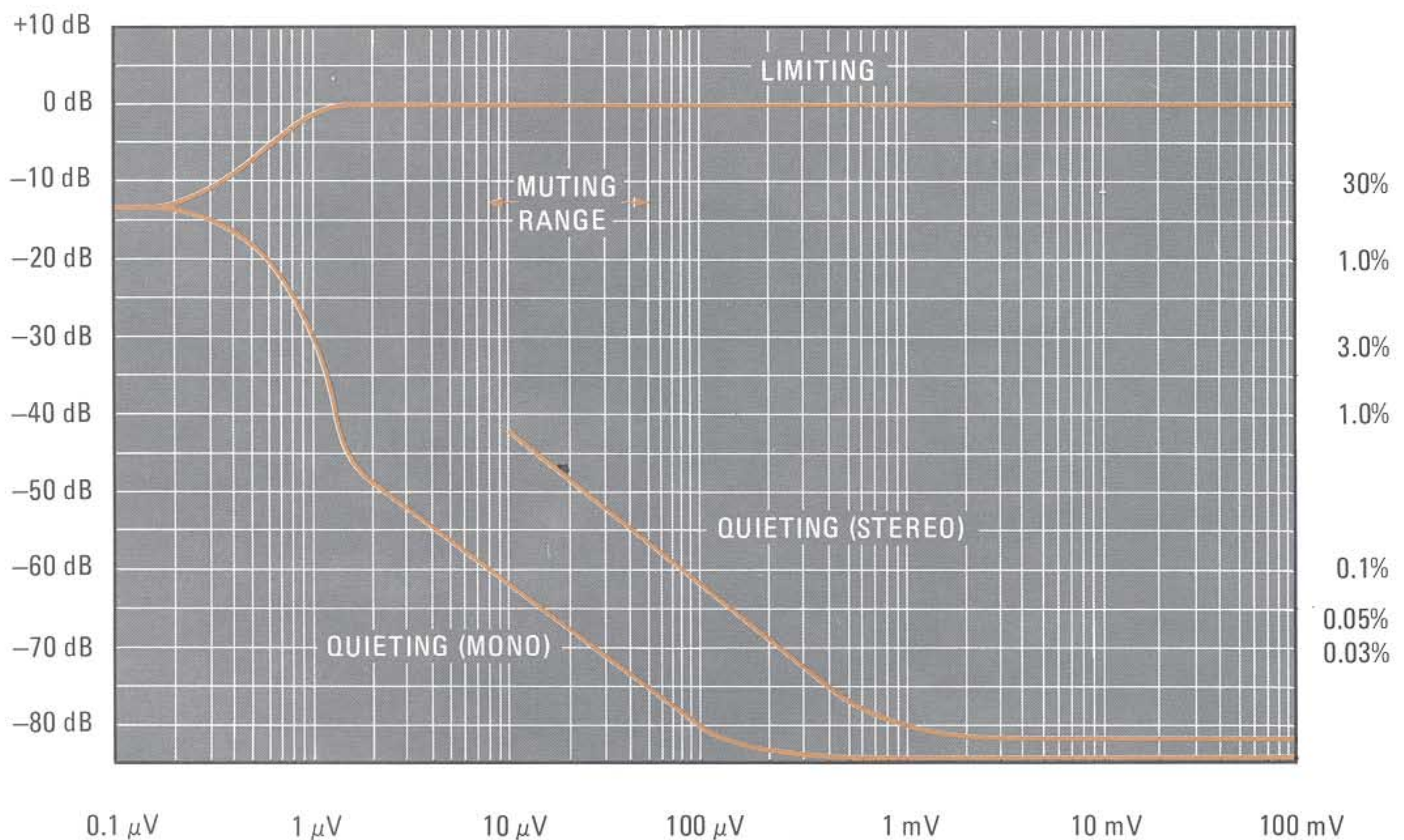
Figure 15. Quieting Slope
