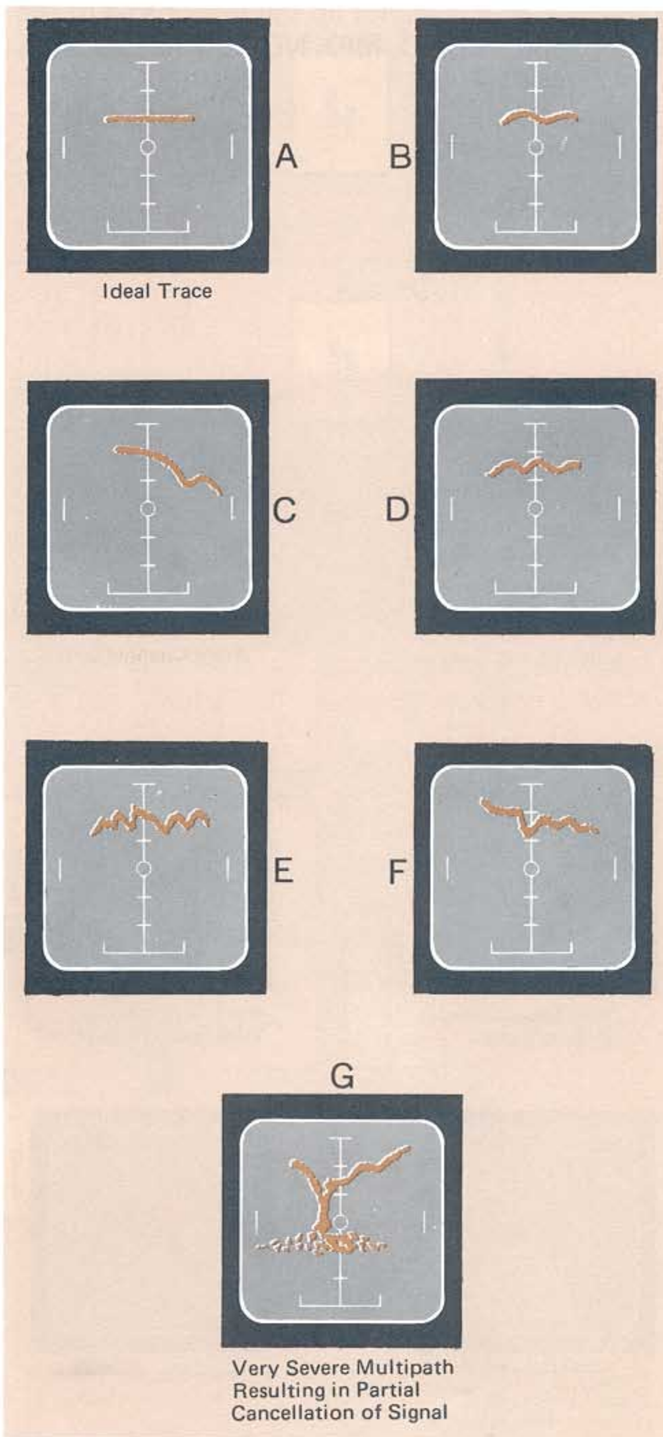
Figure 11. Multipath Distortion Characteristics
