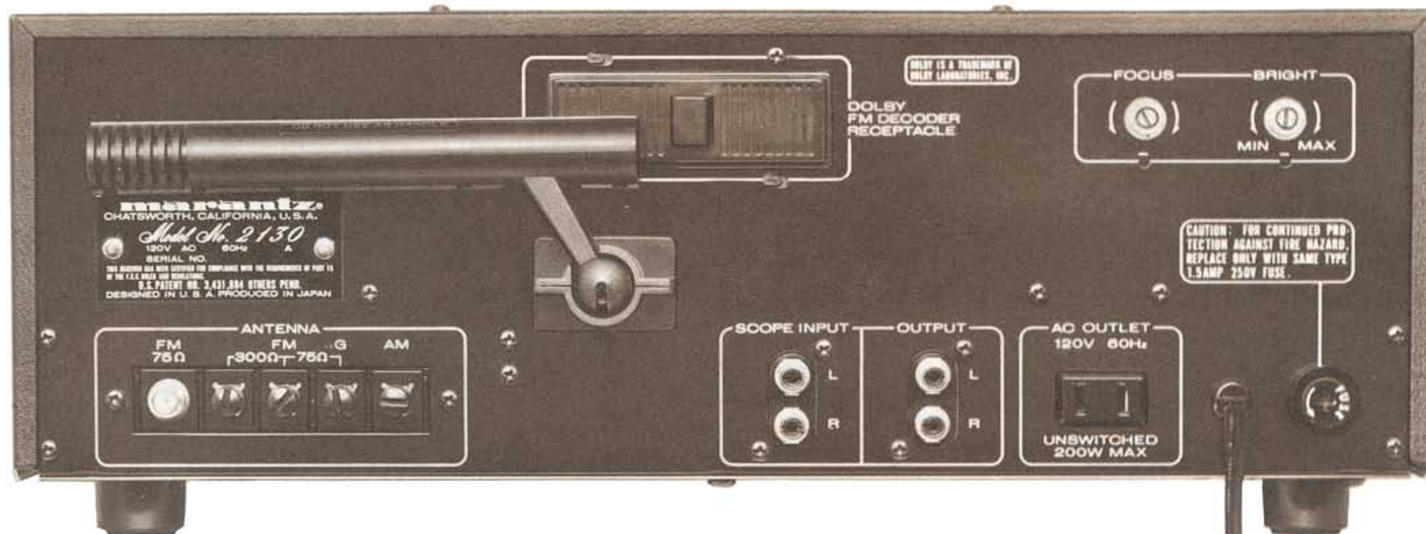
Figure 2. Rear Panel
