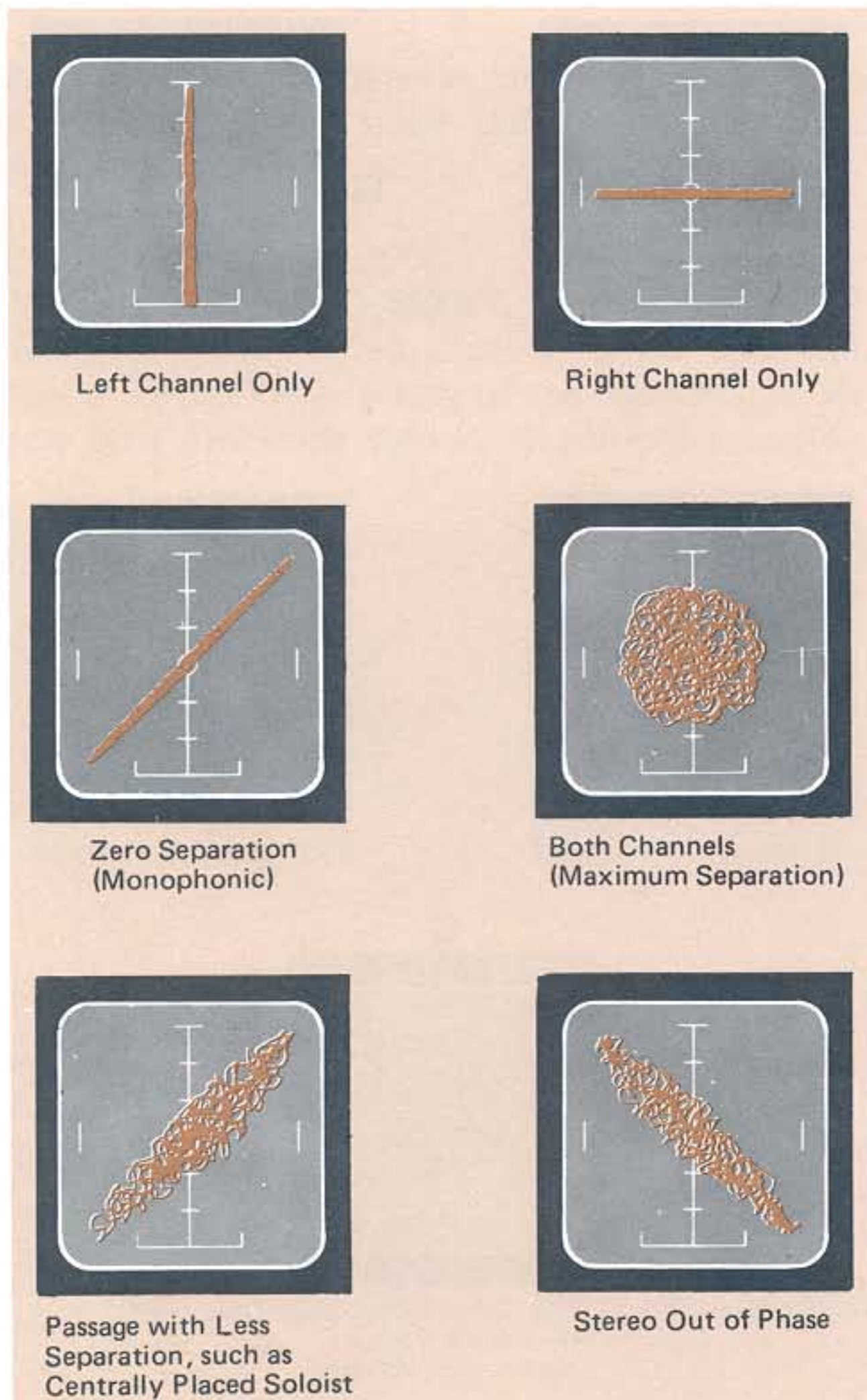
Figure 12. Audio Display
