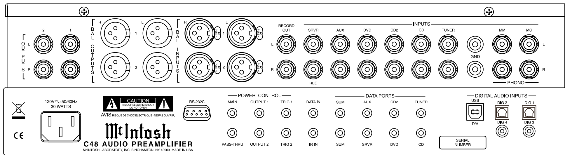
C48 Audio Preamplifier Rear Panel
