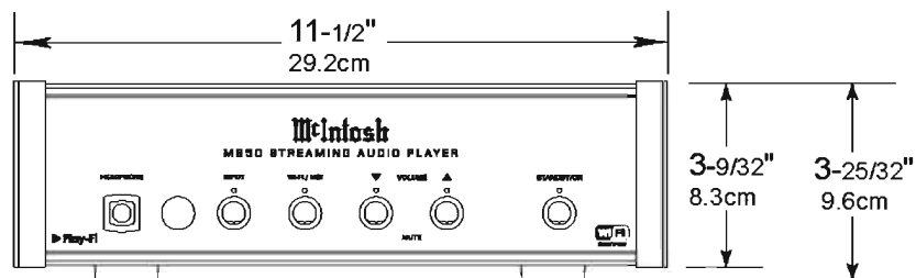
Front View of the MB50
