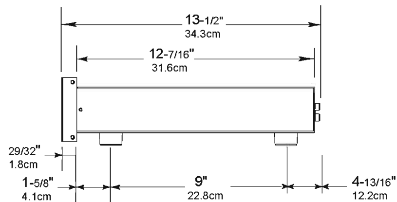
Side View of the MB50
