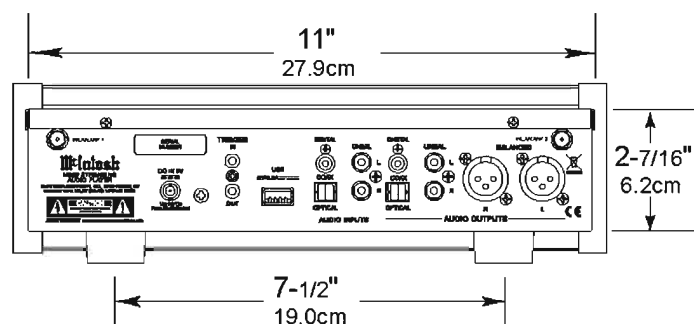
Rear View of the MB50
