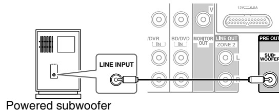
Powered subwoofer
