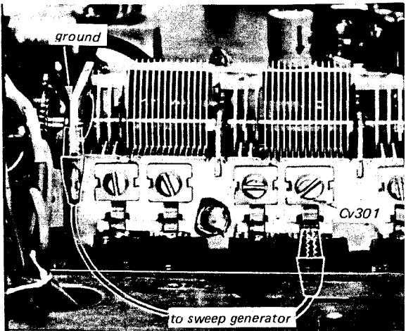
Fig. 3-10 445 kHz sweep signal injection
