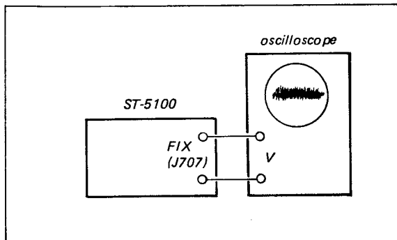
Fig. 3-3 Discriminator alignment test setup
