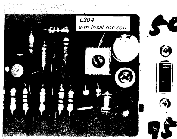
Fig. 3-16 Parts location
