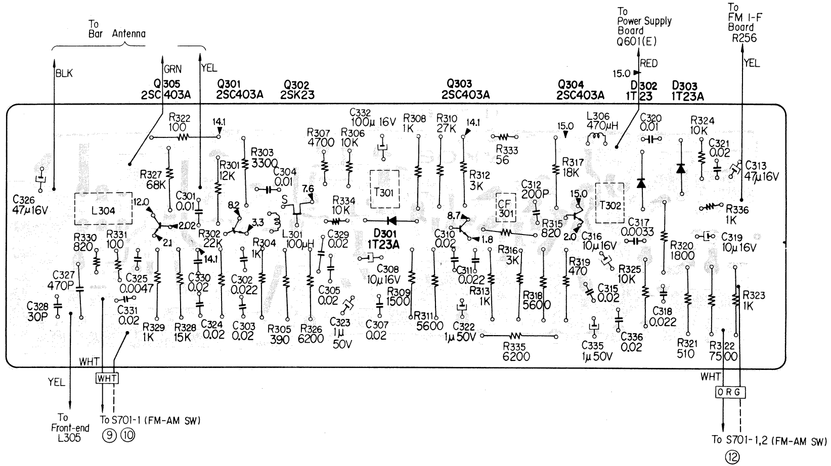
5-3. MOUNTING DIAGRAM—A-m Cp/I-f Board —Conductor Side—
