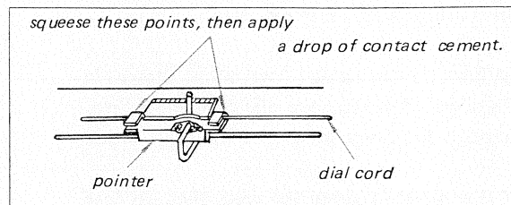
Fig. 2-18 Pointer installation
