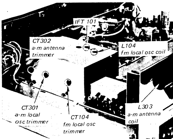
Fig. 3-5 Parts location
