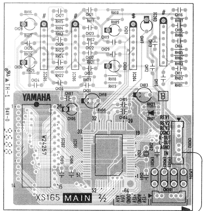
CN301: to DC-CN203 Component side (部品側)
